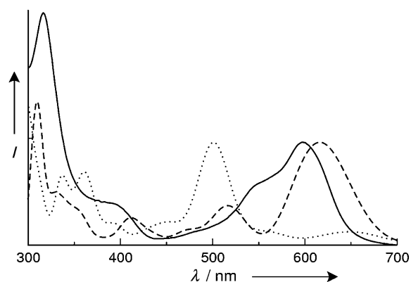
Figure 3. Overlay of experimental absorption spectrum of [\text{Fe}^{\text{II}}(\mathbf{2})_2] (—) with calculated spectra for model complexes 5 (.....) and 6 (---).
